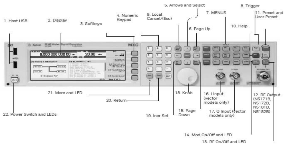
Figura 1. Panel frotar Generador vectorial Keysight N5172B EXG X-Series [1]
