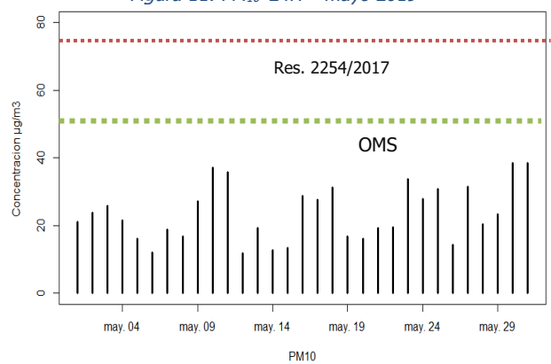
Figura 11: PM10 24H – mayo 2019
