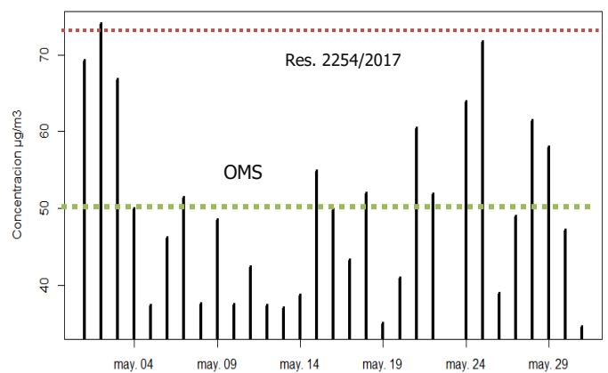
Figura 3: PM10 24H – mayo 2019
