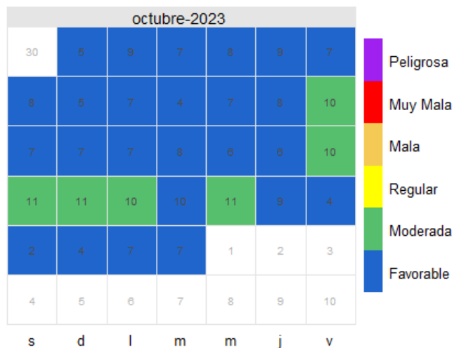
Figura 4. IBOCA pm 10 .
