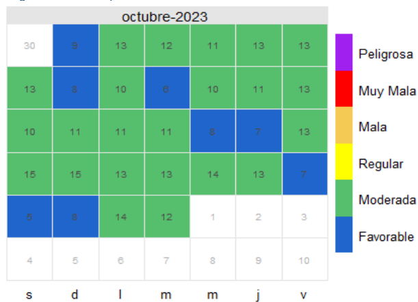
Figura 5. IBOCA pm 2.5
